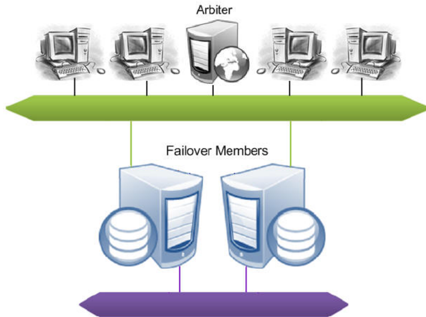
Figure 2–5: Mirror Failover Members and Arbiter
