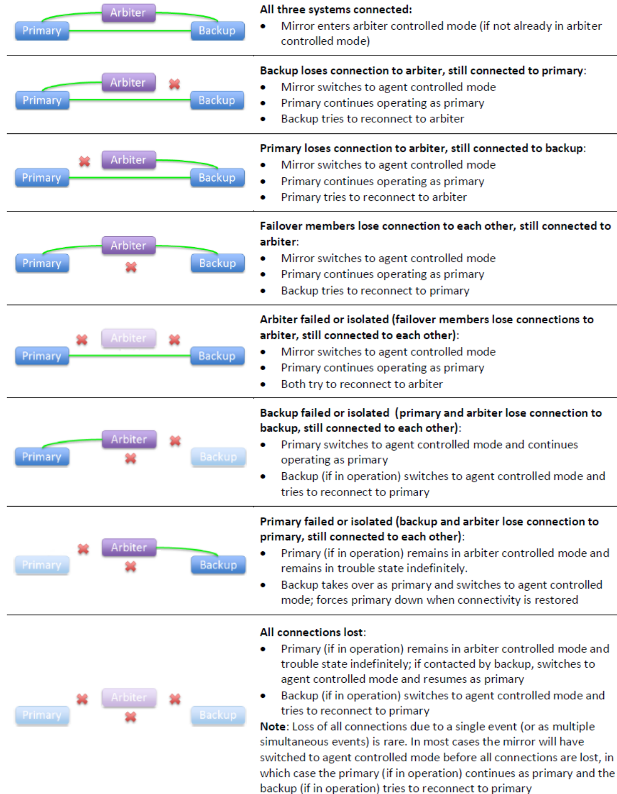
Figure 2–6: Mirror Responses to Lost Connections in Arbiter Mode
