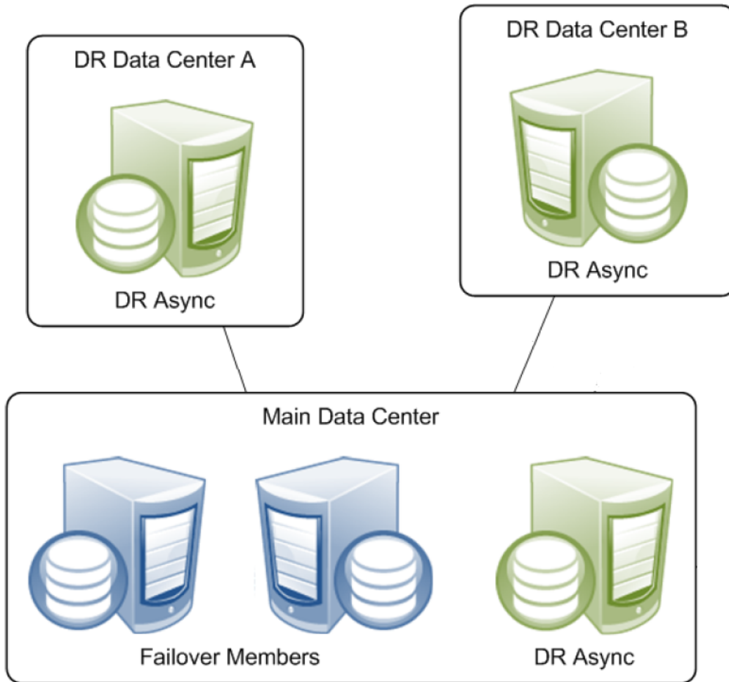
Figure 2-2: Multiple DR Async Members Connected to a Single Mirror
