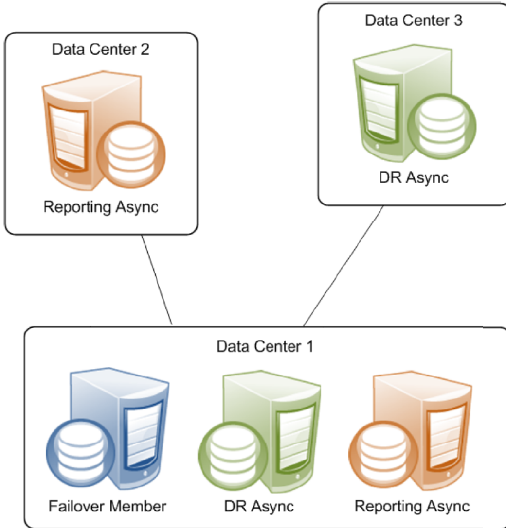
Figure 2–4: Single Failover Member with Multiple Async Members
