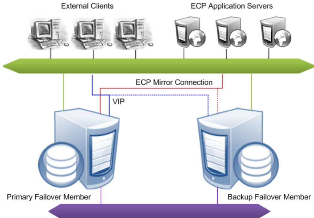
Figure 2–1: Mirror Failover Members
