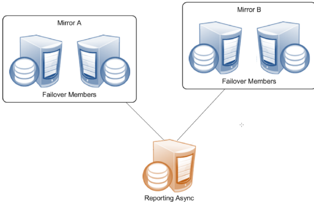
Figure 2–3: Single Reporting Async Member Connected to Multiple Mirrors
